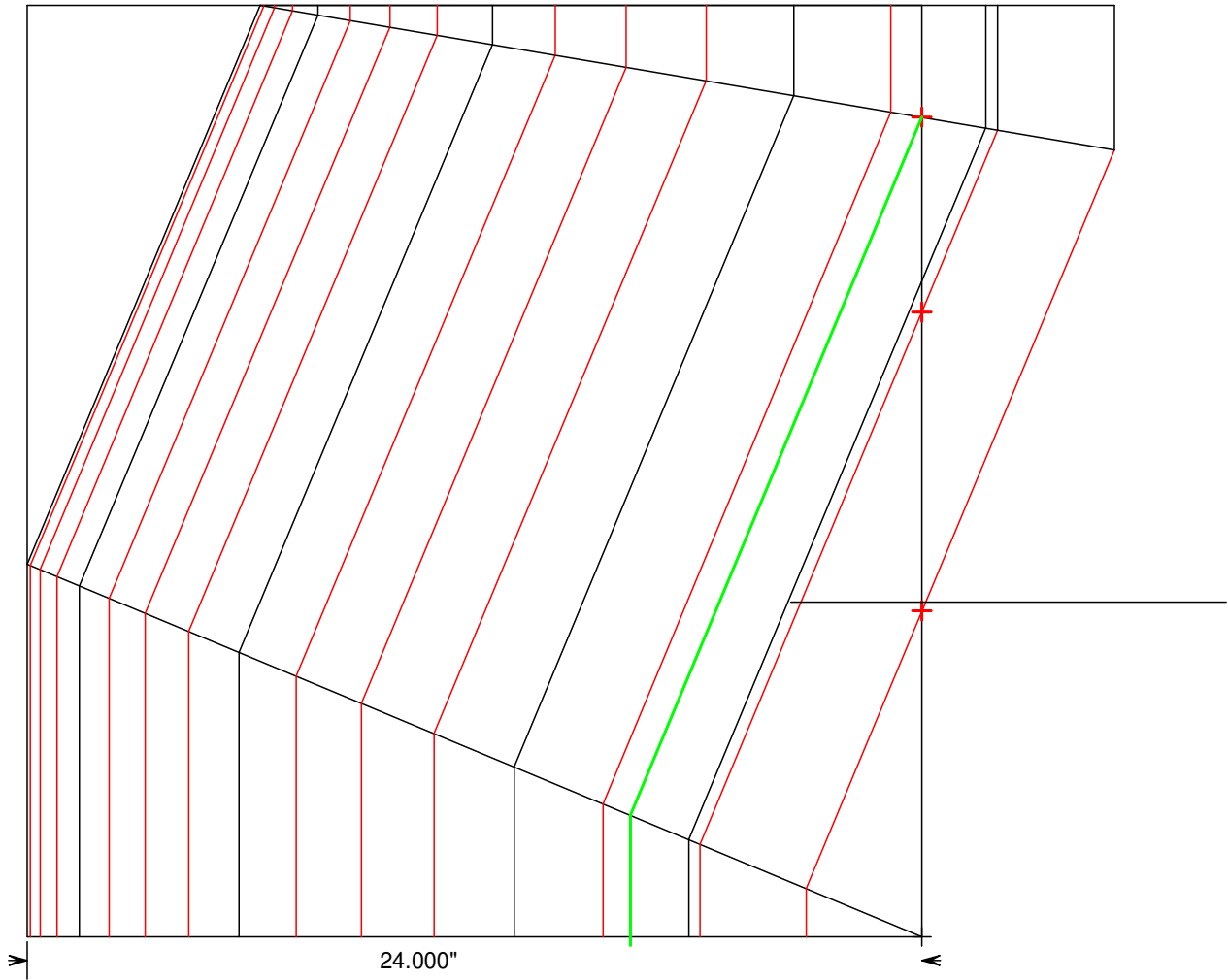
Chine And Sheer Body View of Fig 3.1-3.3
